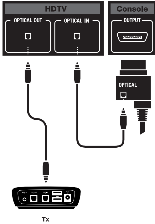
XBOX 360 (Original)
